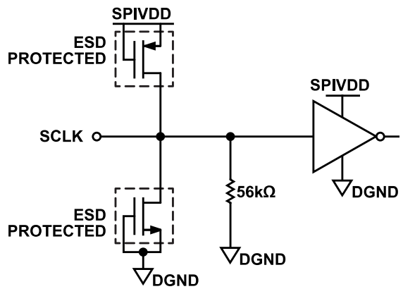
Figure 46. SCLK Input
