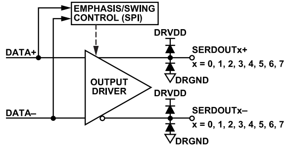
Figure 44. Digital Outputs
