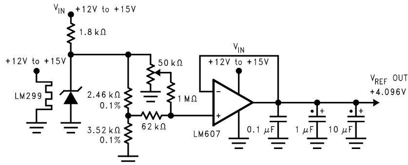
Figure 70. Low Drift Extremely Stable Reference Circuit
