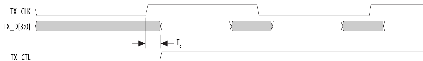
Figure 14. RGMII TX Timing Diagram
