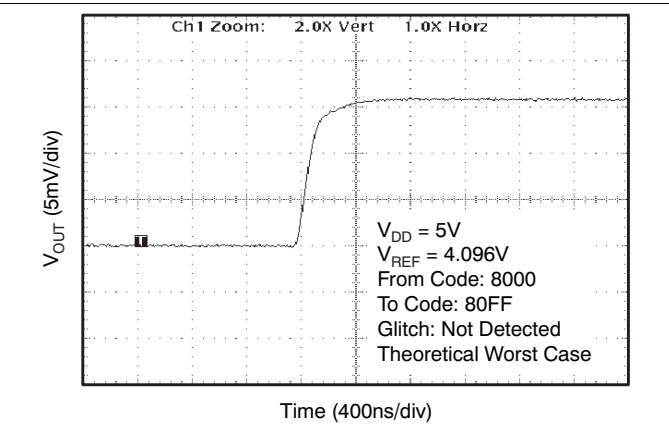
Figure 21. Glitch Energy: 5-V, 256-LSB Step, Rising Edge
