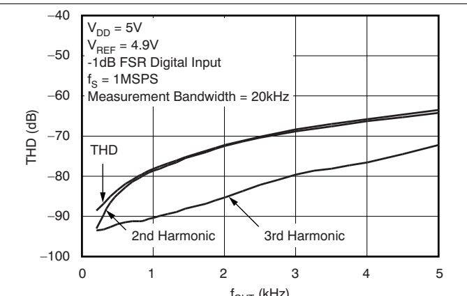
Figure 23. Total Harmonic Distortion vs Output Frequency
