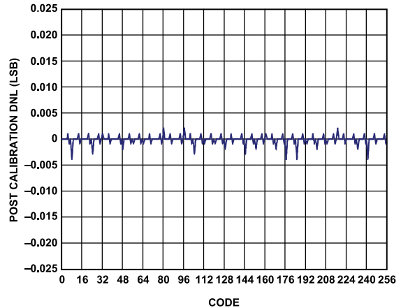
Figure 39. AD9714 Postcalibration DNL at 3.3 V
