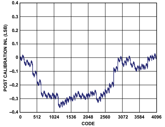
Figure 21. AD9716 Postcalibration INL at 3.3 V
