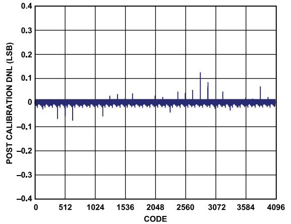
Figure 22. AD9716 Postcalibration DNL at 3.3 V
