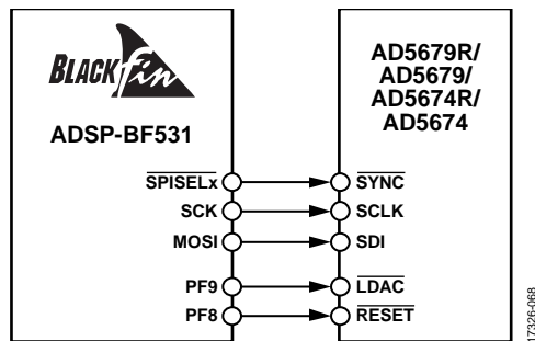
Figure 68. ADSP-BF531 Interface
