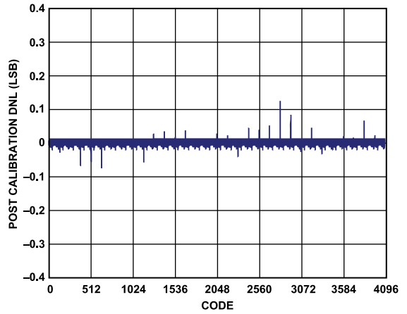
Figure 22. AD9716 Postcalibration DNL at 3.3 V
