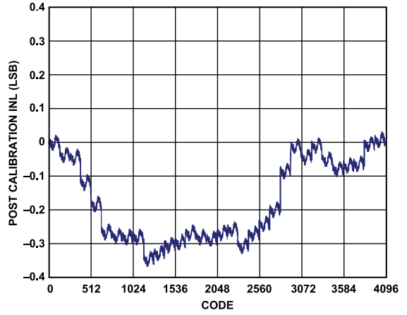
Figure 21. AD9716 Postcalibration INL at 3.3 V
