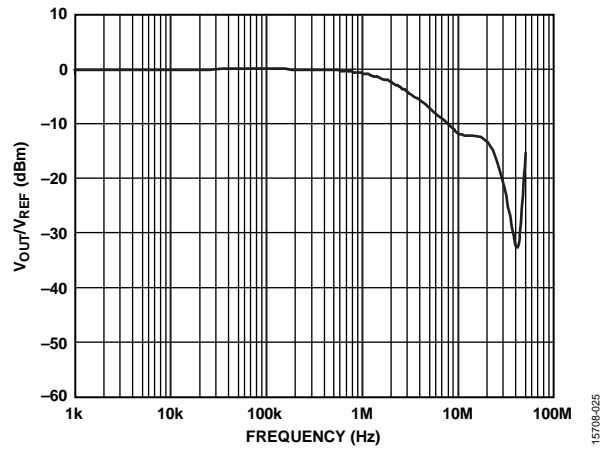
Figure 25. Multiplying Bandwidth
