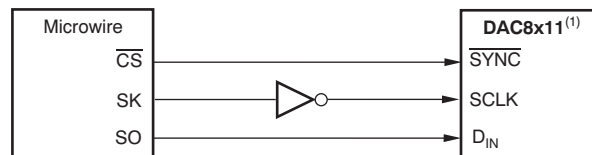
Figure 82. DAC8x11 to Microwire Interface
