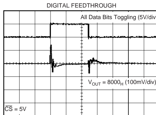
Time (200ns/div)
