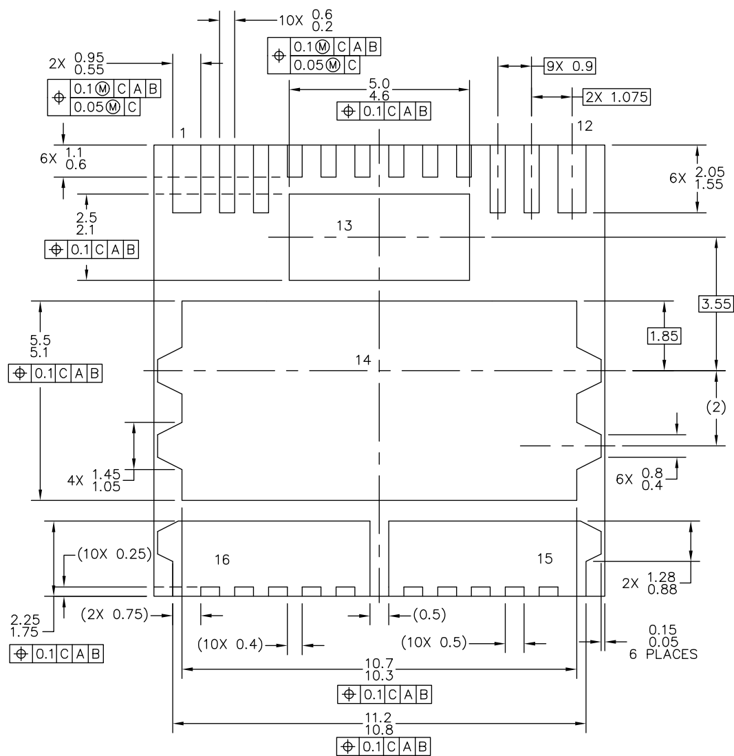
VIEW M-M
