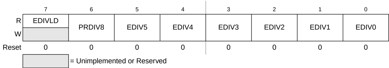
Figure 4-4. EEPROM Clock Divider Register (ECLKDIV)
