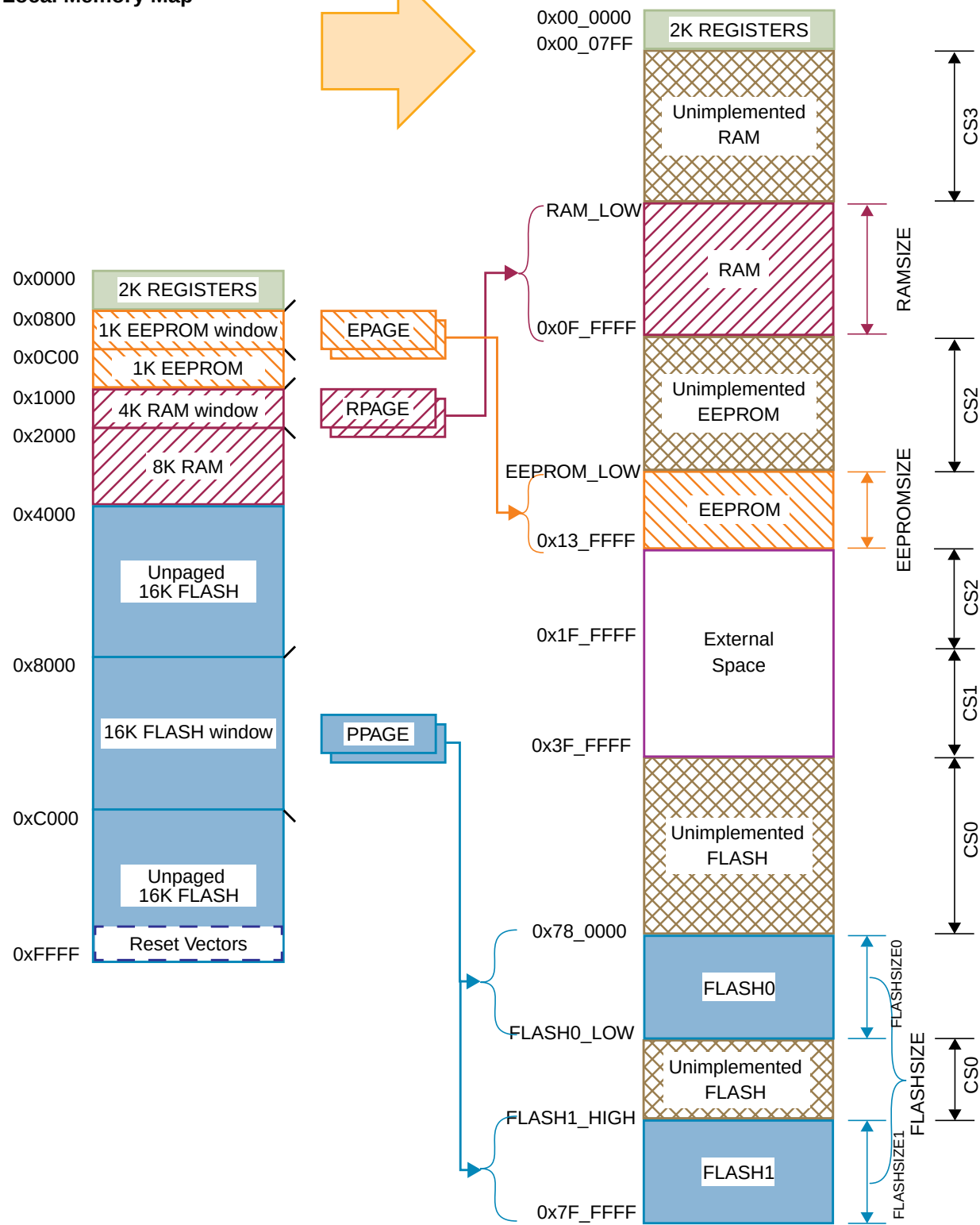
Figure 1-2. MC9S12XHZ Family Global Memory Map
