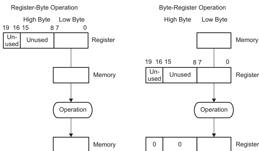
Figure 6-10. Register-Byte and Byte-Register Operation
