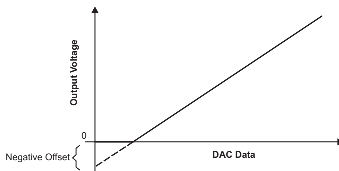
Figure 31-5. Negative Offset
