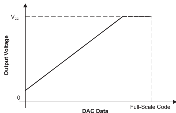
Figure 31-6. Positive Offset
