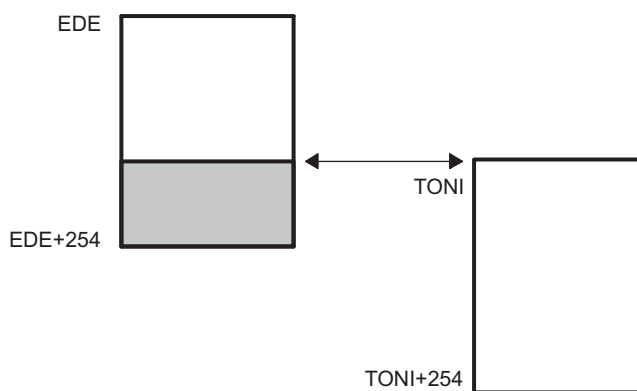
Figure 6-36. Decrement Overlap
