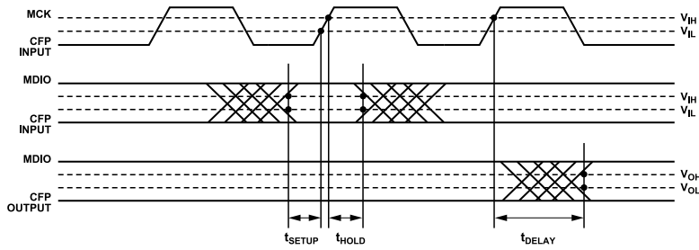
Figure 7. MDIO Timing
