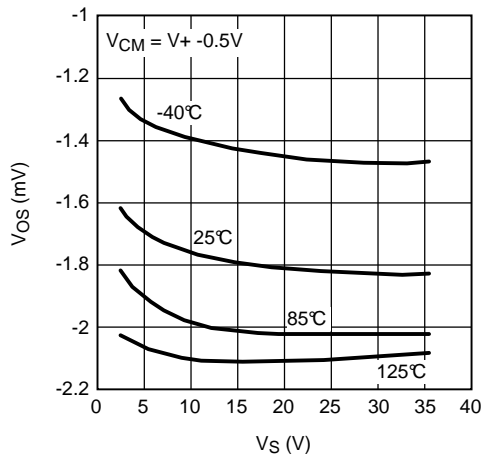
Figure 22. V_{OS} vs. V_S (Unit 3)
