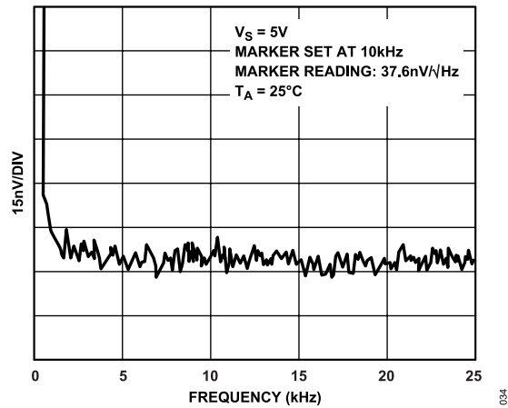
Figure 35. Voltage Noise
