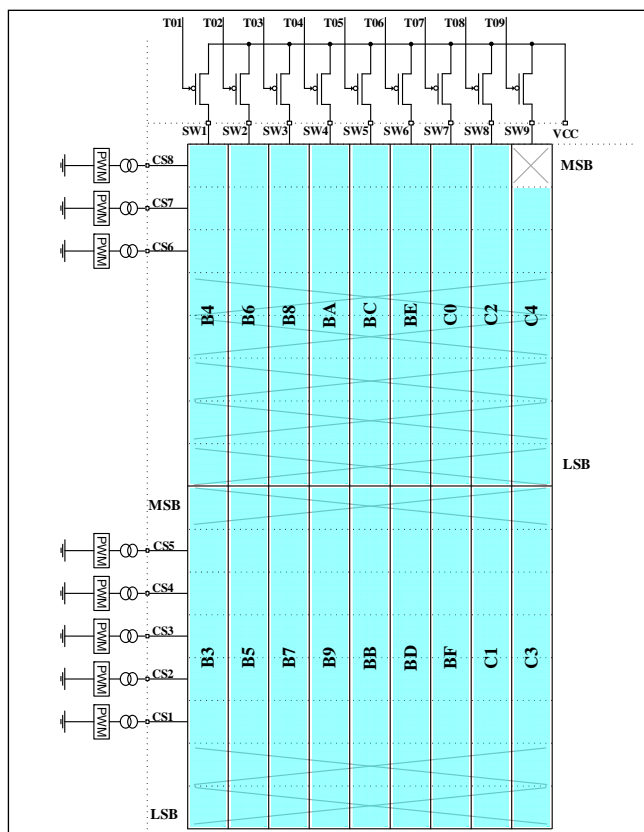
Figure 11 Open/Short Register
