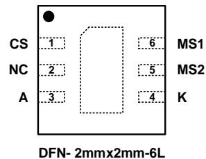
DFN- 2mmx2mm-6L
