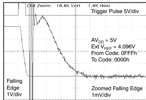
Time (2μs/div)
