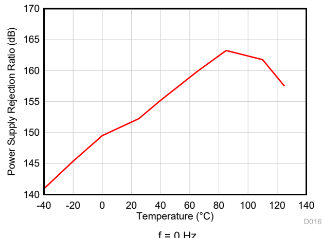
Figure 6-18. PSRR vs Temperature (dB)
