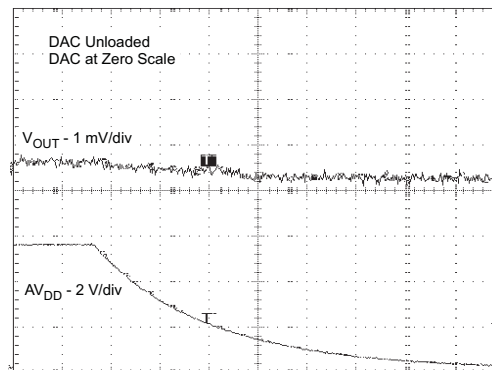
POWER-OFF GLITCH
