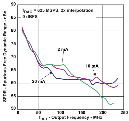
Figure 6. SFDR vs I_{OUTFS}
