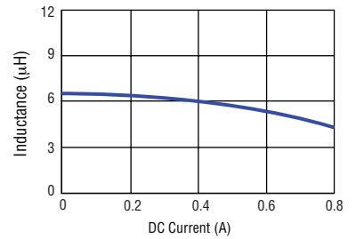
SRN2009T-6R8M
