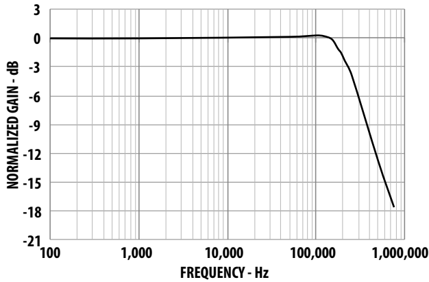
Figure 17: Gain Frequency Response
