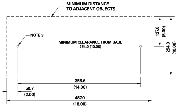
MOUNTING DETAIL
