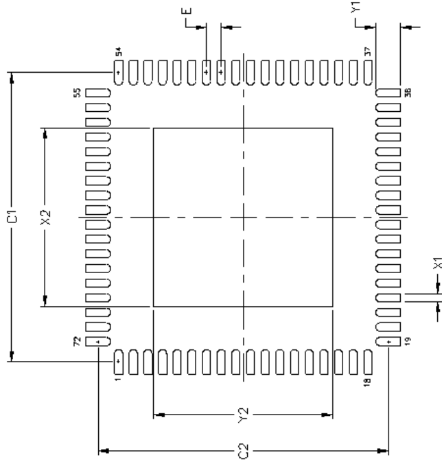
Figure 14. 72-Pin Quad Flat No Lead (QFN) Package
