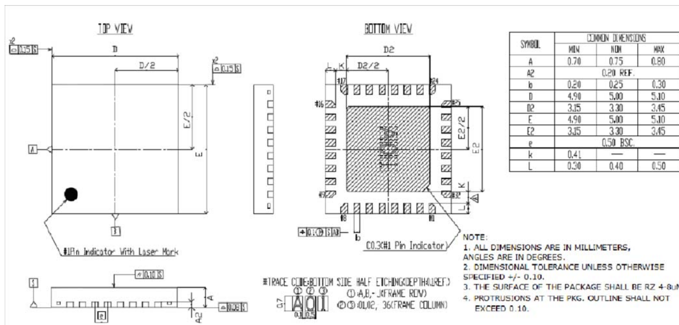
32-Lead QFN 5x 5mm
