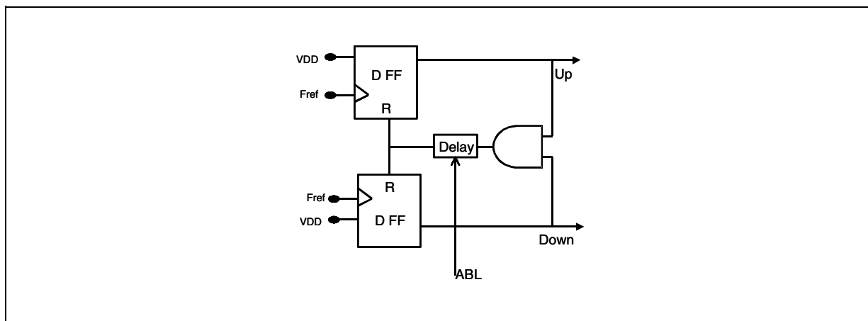
Figure 14. PFD Diagram
