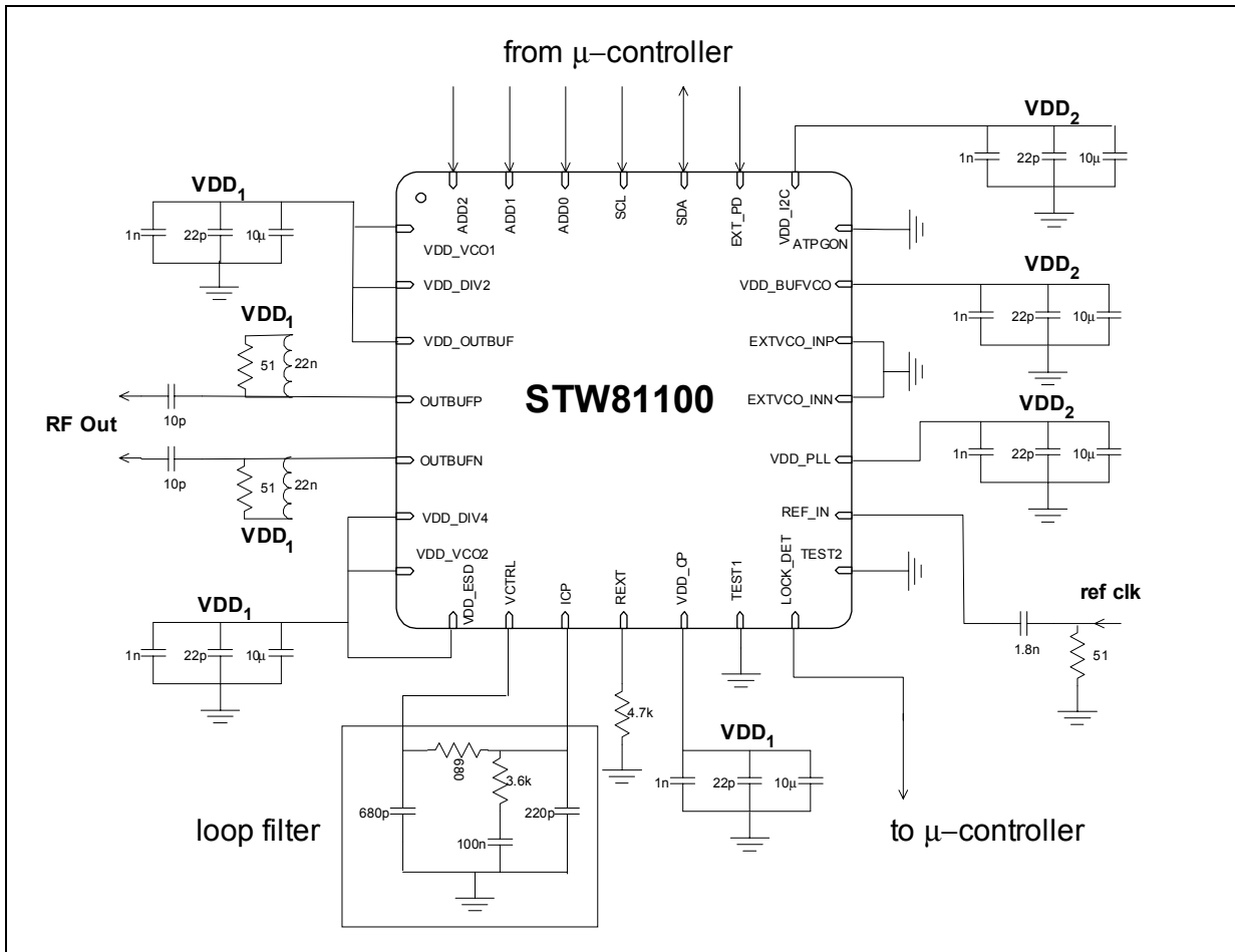
Figure 31. Application diagram
