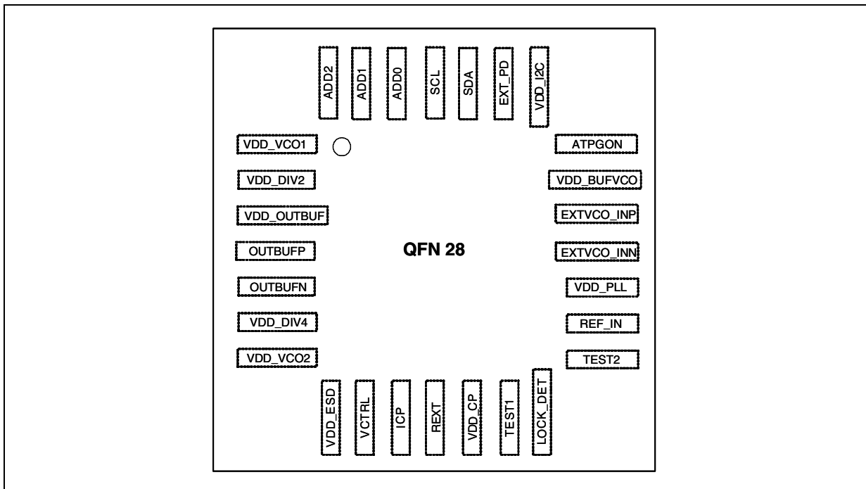
Figure 3. Pin Connections
