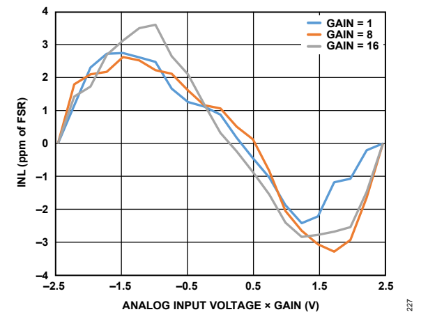
Figure 27. INL vs. Differential Input Signal (Analog Input x Gain), ODR = 50 SPS, Internal Reference
