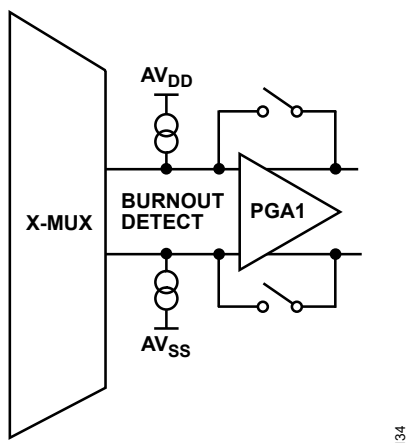
Figure 124. Burnout Currents
