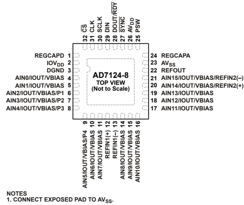
Figure 9. Pin Configuration
