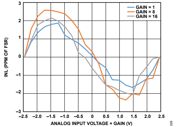
Figure 26. INL vs. Differential Input Signal (Analog Input x Gain), ODR = 50 SPS, External 2.5 V Reference
