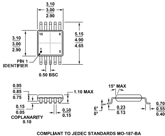
Figure 49. 10-Lead Mini Small Outline Package [MSOP] (RM-10) Dimensions shown in millimeters
