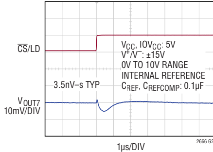
DAC-to-DAC Crosstalk
