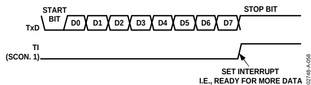
Figure 51. UART Serial Port Transmission, Mode 1
