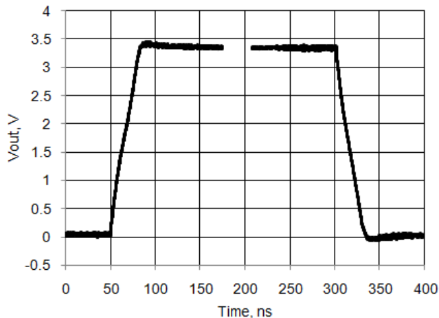
Figure 11-8. GPIO Output Rise and Fall Times, Slow Strong Mode, V DDIO = 3.3 V, 25 pF Load
