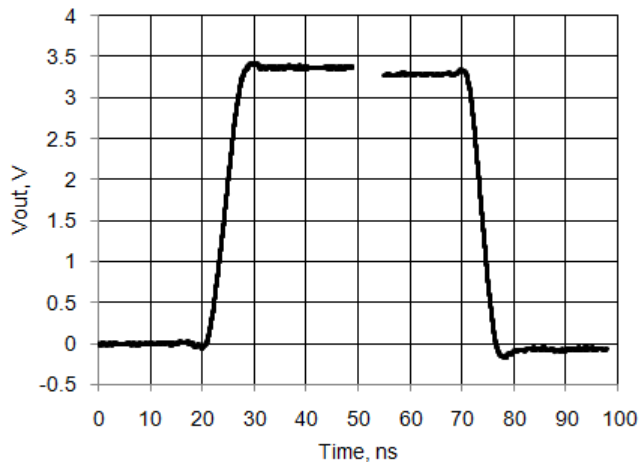
Figure 11-16. USBIO Output Rise and Fall Times, GPIO Mode, V_{\text{DDD}} = 3.3\text{ V} , 25 pF Load
