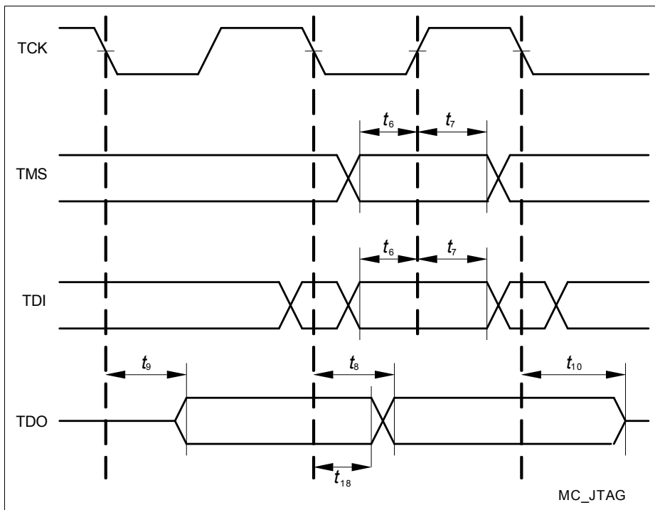
Figure 27 JTAG Timing
