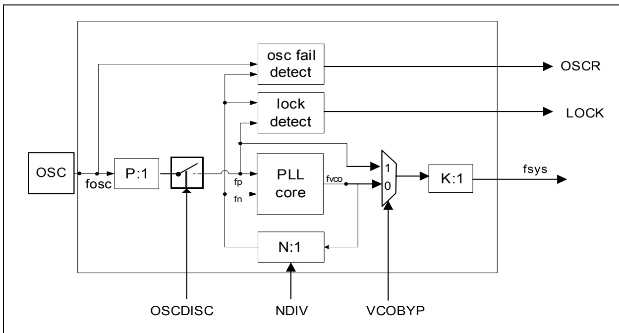
Figure 22 CGU Block Diagram
