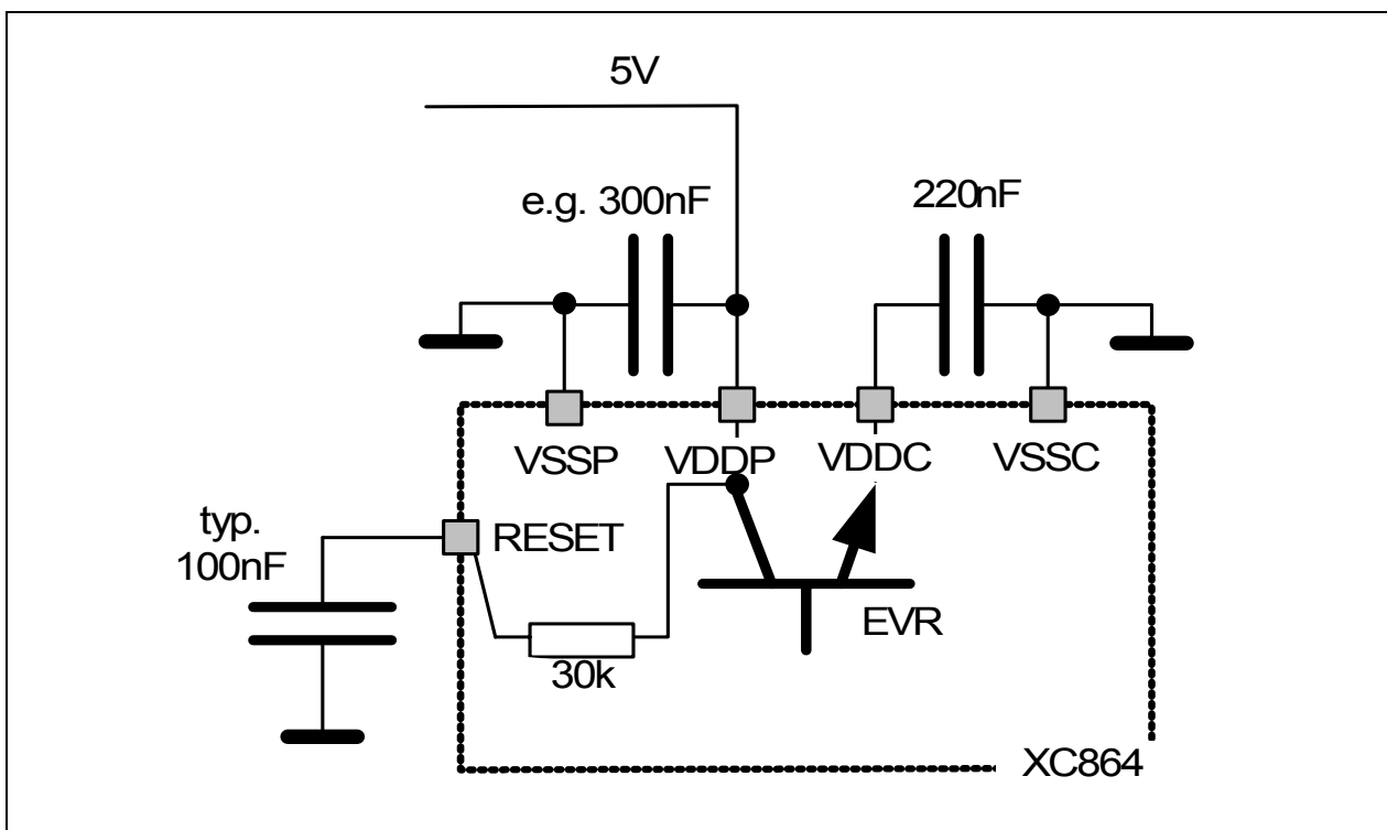
Figure 20 Reset Circuitry
