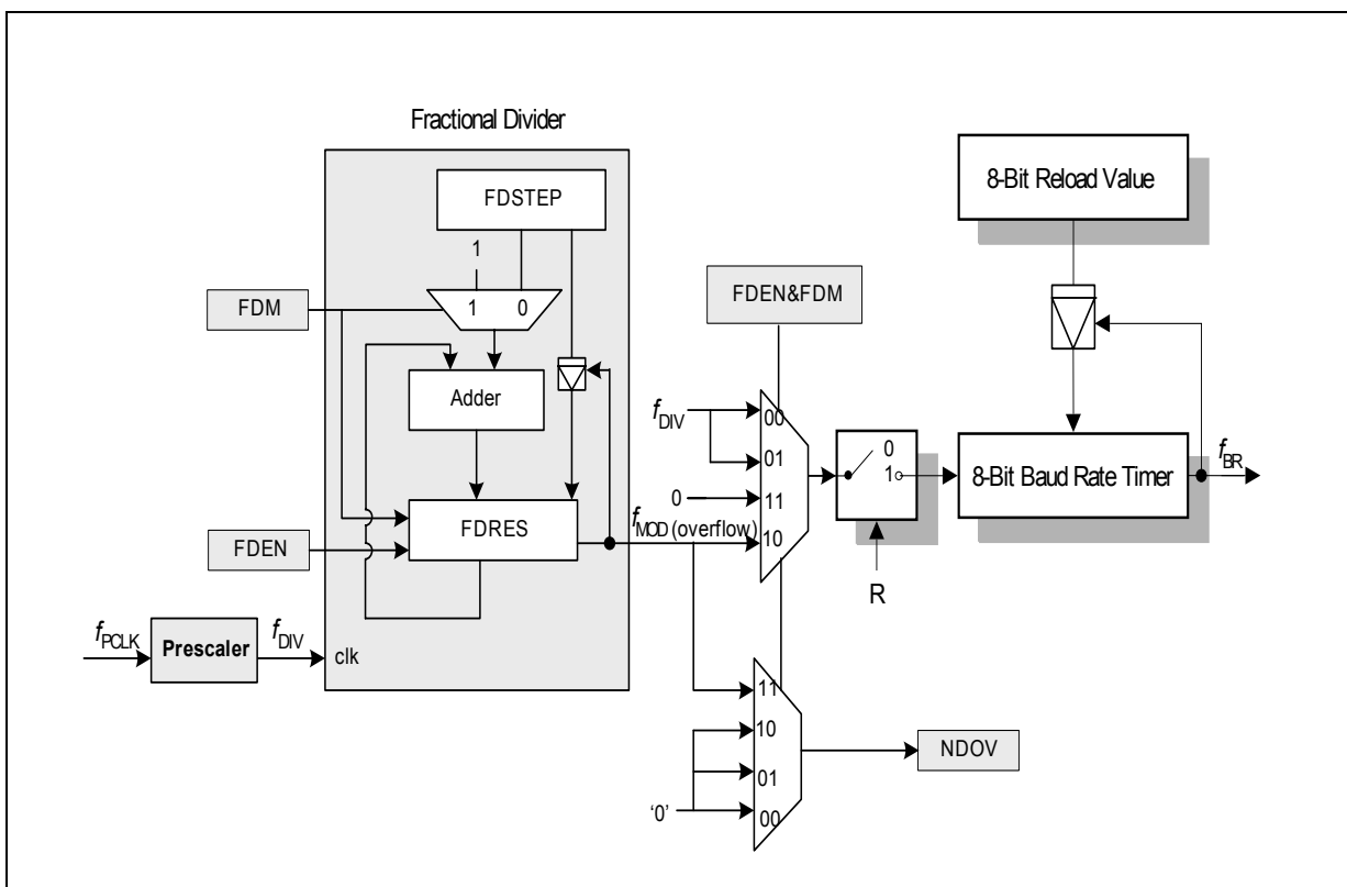
Figure 27 Baud-rate Generator Circuitry
