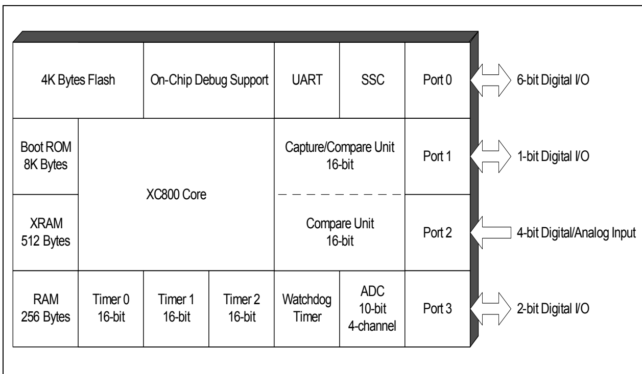
Figure 1 XC864 Functional Units
