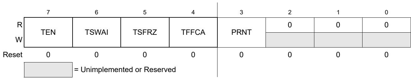
Figure 23-12. Timer System Control Register 1 (TSCR1)
