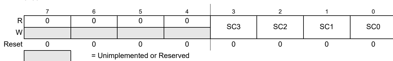
Figure 8-11. Debug State Control Register 3 (DBGSCR3)
