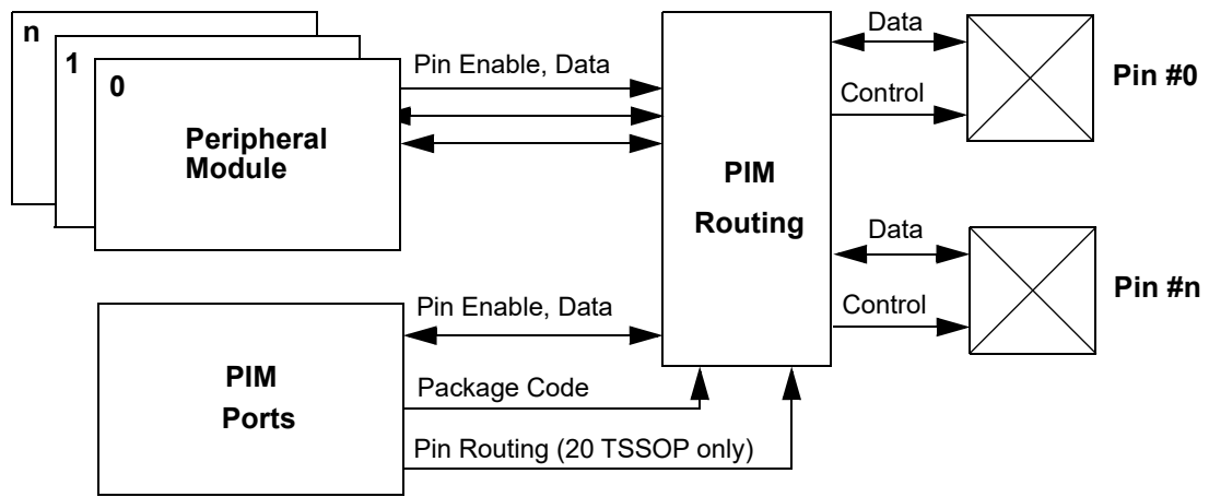
Figure 2-1. Block Diagram
