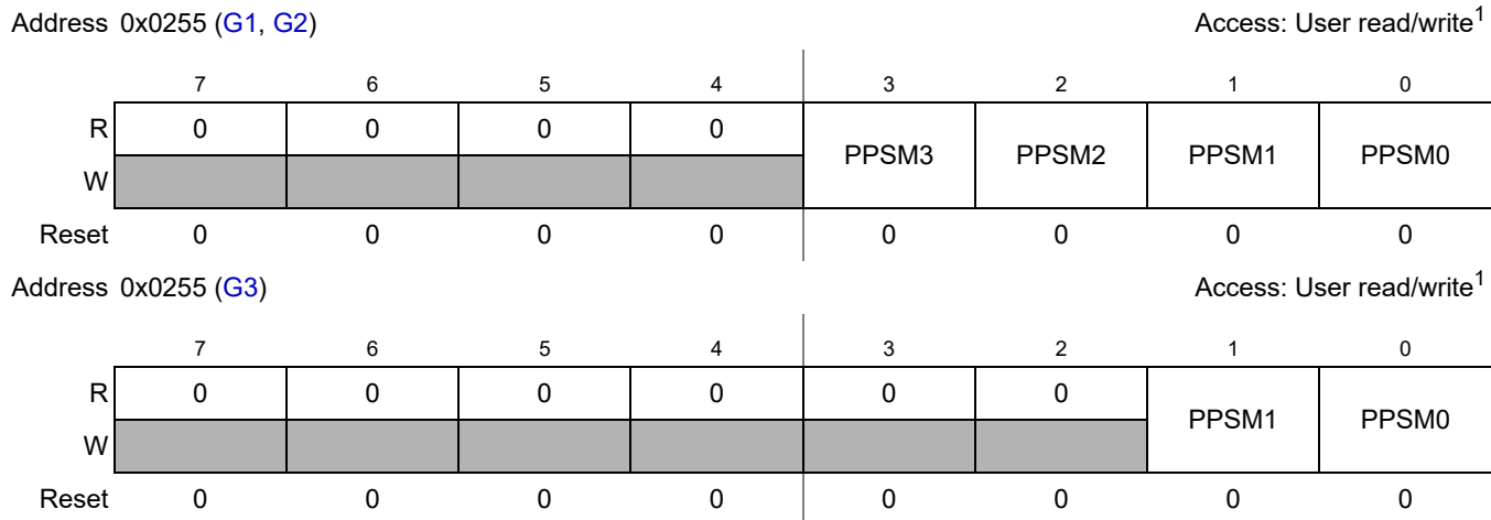
Figure 2-32. Port M Polarity Select Register (PPSM)
