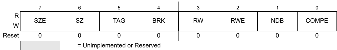
Figure 8-13. Debug Comparator Control Register DBGACTL (Comparator A)
