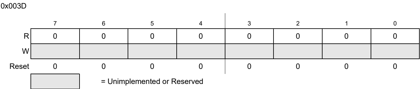
Figure 10-13. Reserved Register (CPMUTEST0)
