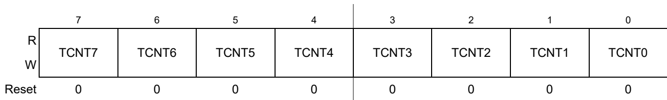
Figure 23-11. Timer Count Register Low (TCNTL)
