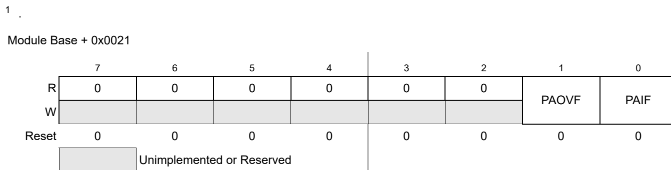
Figure 23-25. Pulse Accumulator Flag Register (PAFLG)
