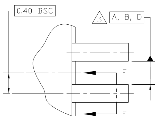
DETAIL G
