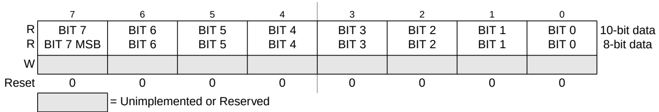
Figure 5-18. Right Justified, ATD Conversion Result Register, Low Byte (ATDDRxL)
