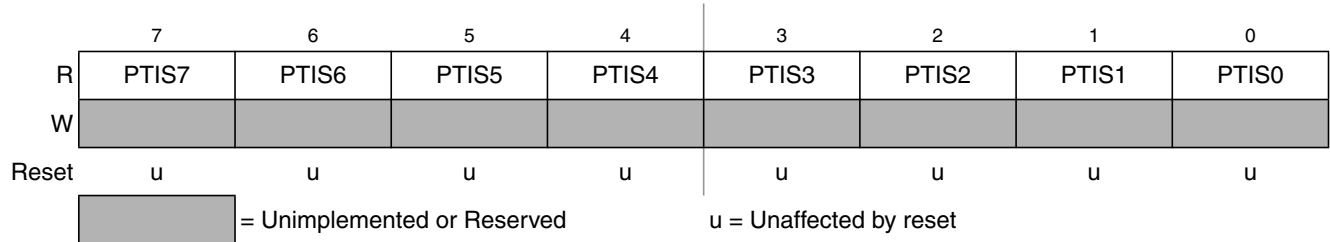
Figure 2-28. Port S Input Register (PTIS)
