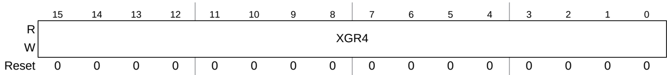
Figure 5-15. XGATE Register 4 (XGR4)
