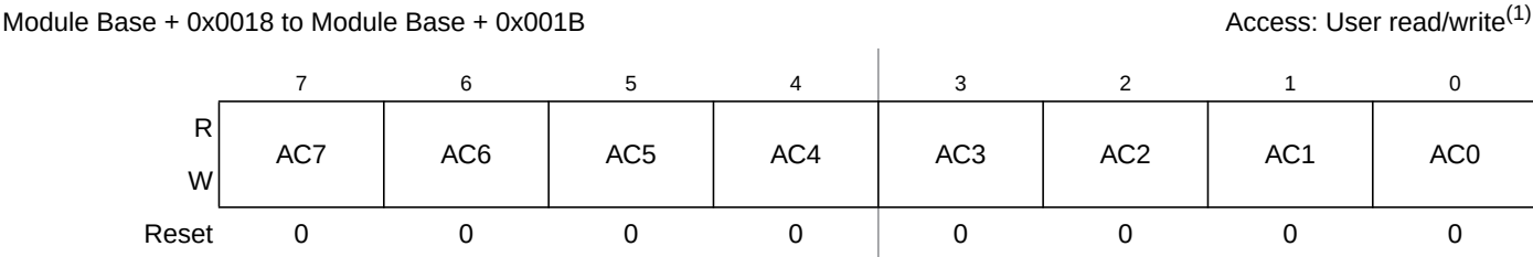
Figure 14-21. MSCAN Identifier Acceptance Registers (Second Bank) — CANIDAR4–CANIDAR7
