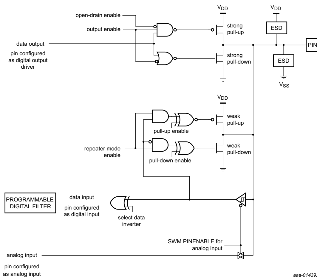
Fig 9. Standard I/O pad configuration
