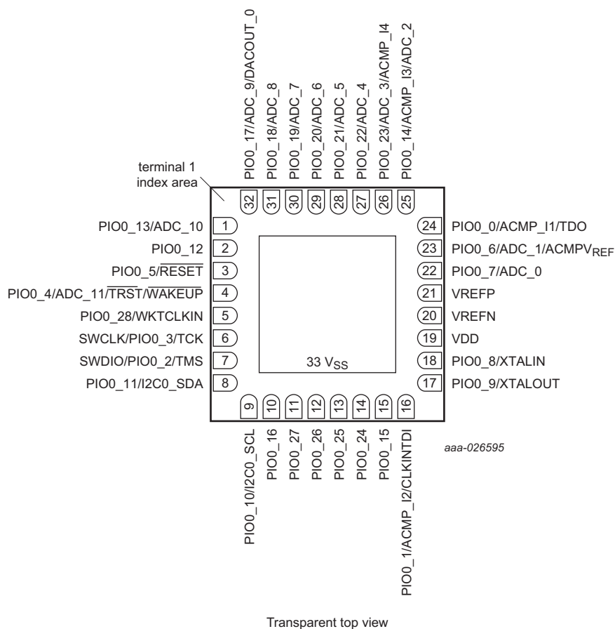
Fig 7. Pin configuration HVQFN33 package
