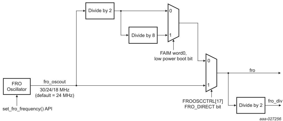
Fig 13. LPC84x FRO subsystem
