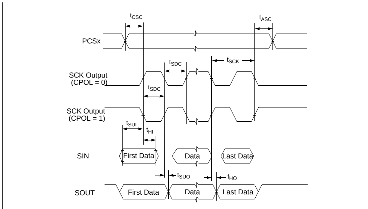
Figure 32. DSPI CMOS master mode – modified timing, \text{CPHA} = 0
