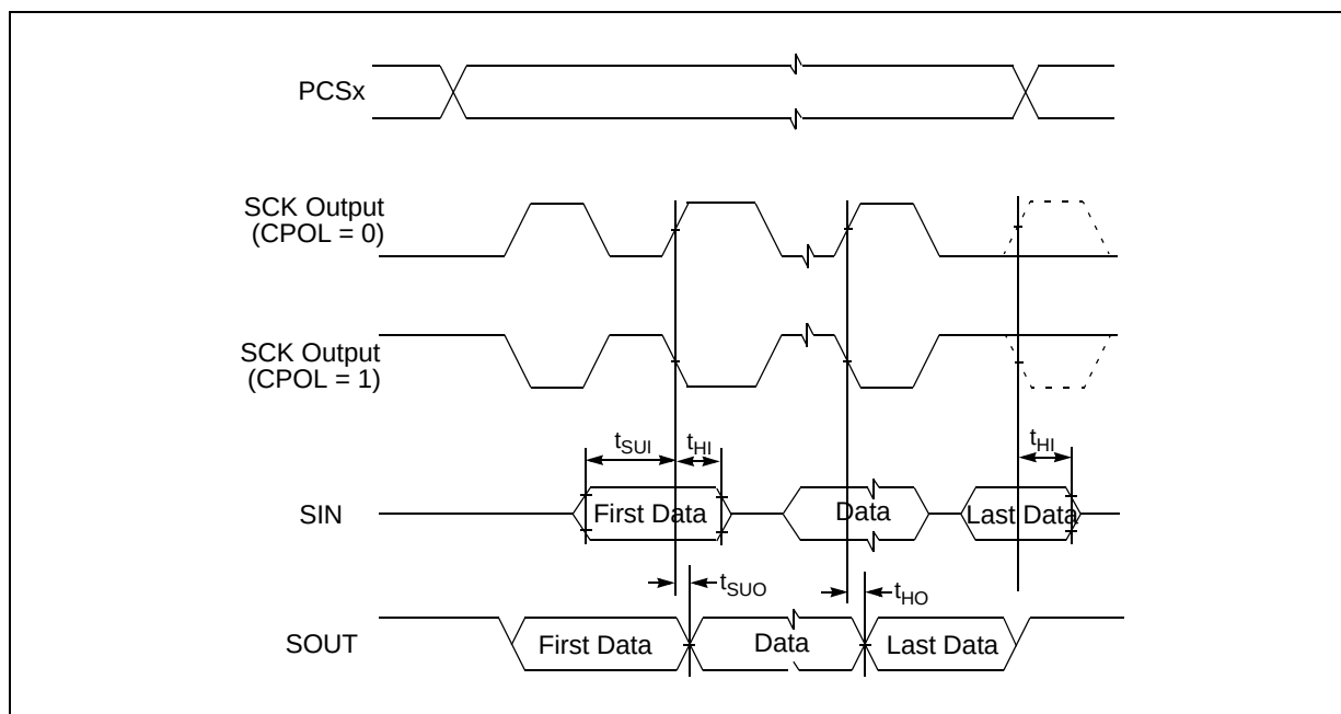
Figure 33. DSPI CMOS master mode – modified timing, \text{CPHA} = 1
