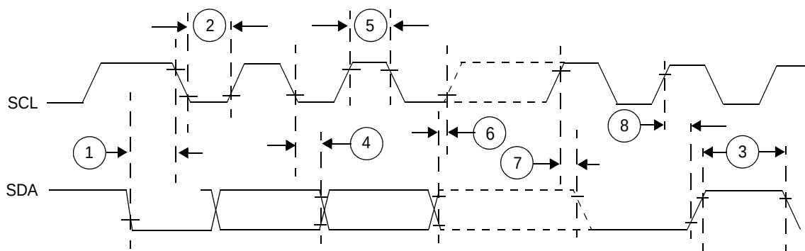
Figure 53. I²C input/output timing
