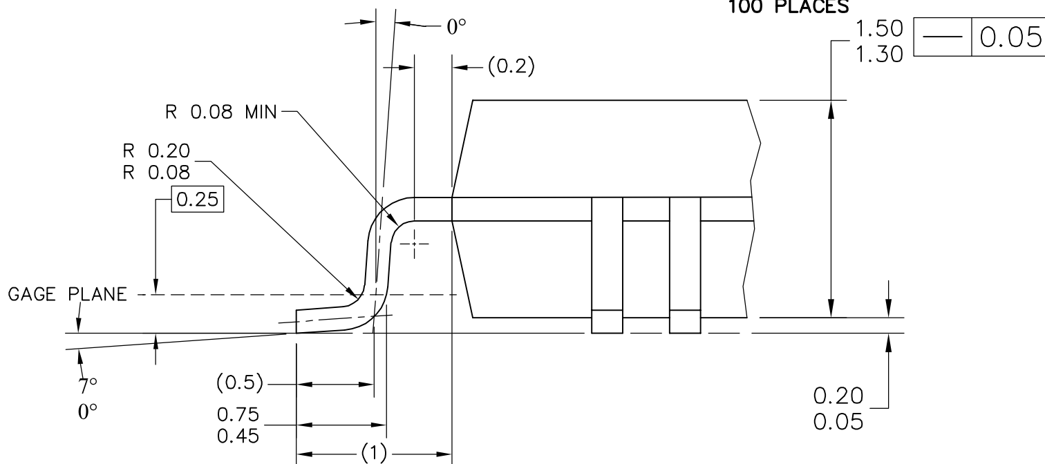
VIEW B
