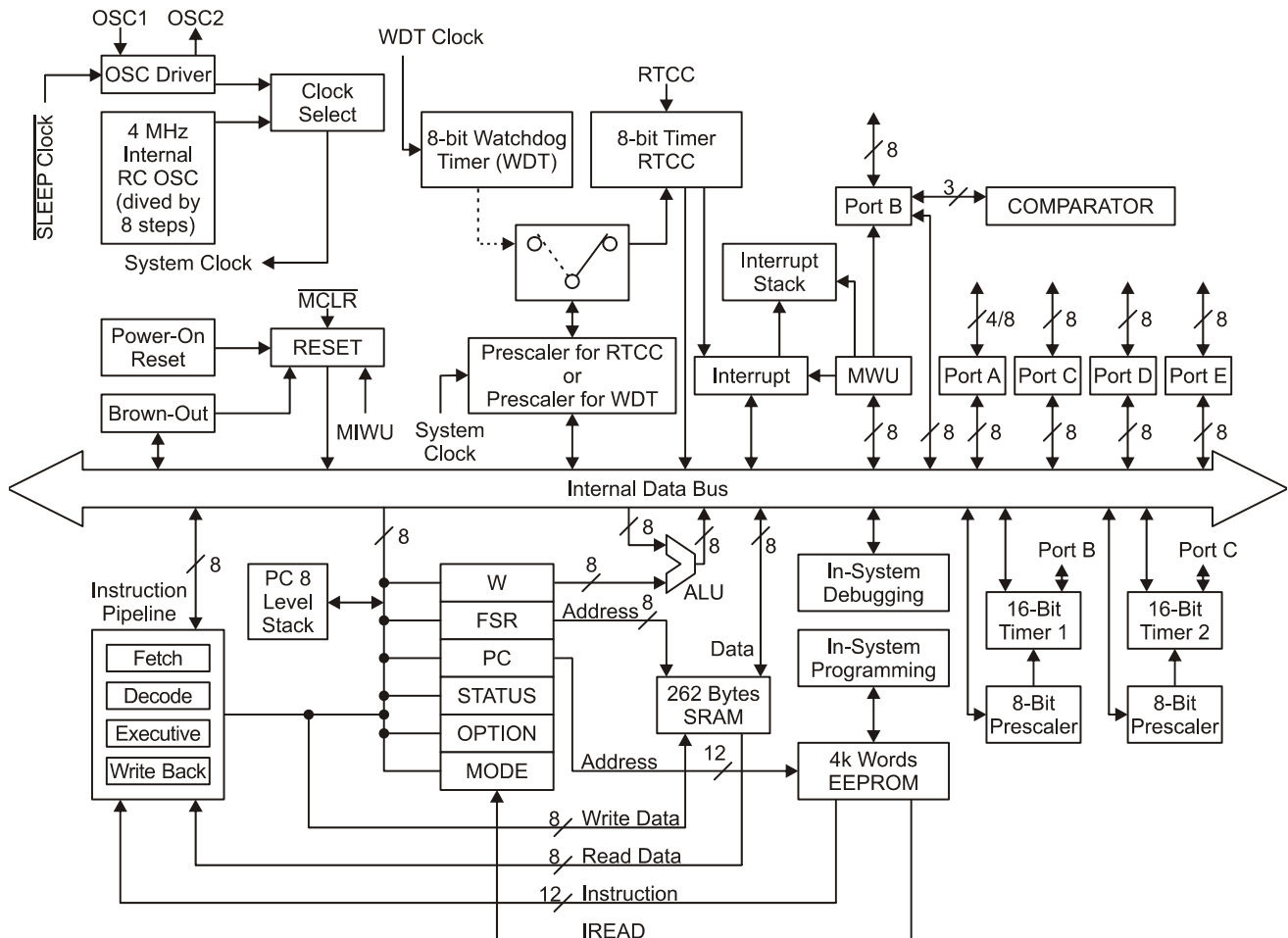
Figure 1-1: Block Diagram
