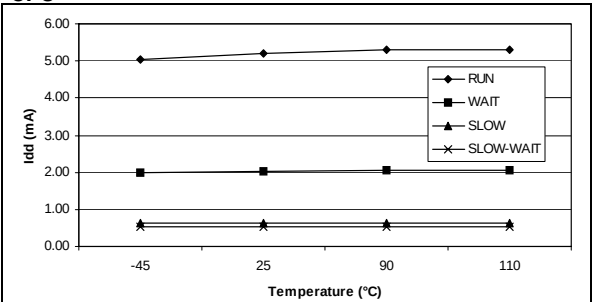
Figure 92. Typical I_{DD} vs. Temp. at V_{DD} = 5\text{V} and f_{CPU} = 8\text{MHz}
