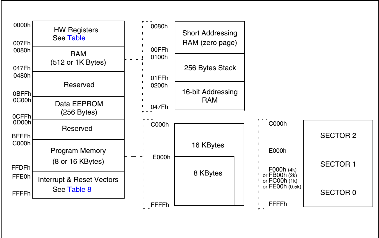
Figure 5. Memory Map
