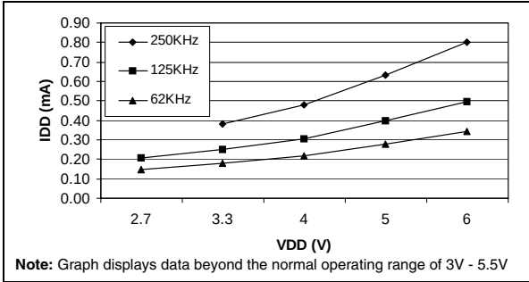
Figure 88. Typical I_{DD} in SLOW vs. f_{CPU}
