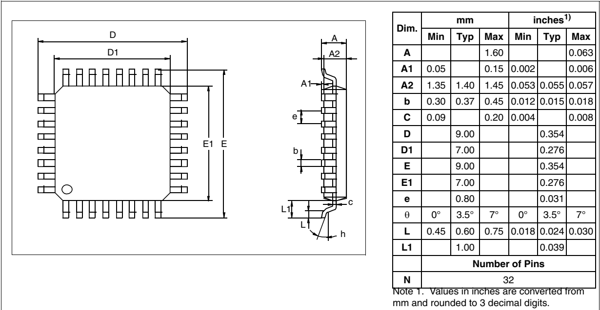
Figure 116. 32-Pin Low Profile Quad Flat Package (7x7)
