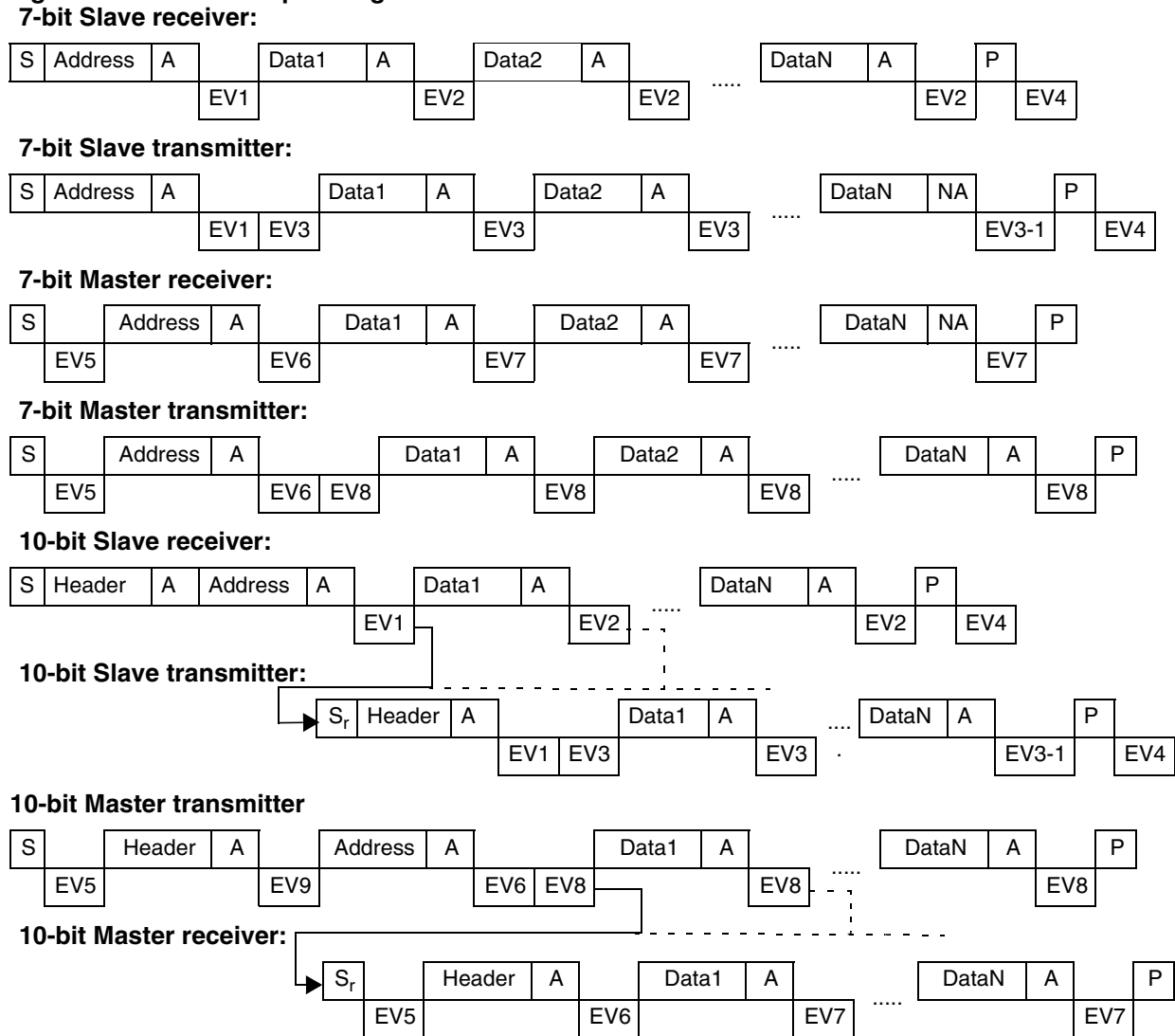
Figure 66. Transfer Sequencing
