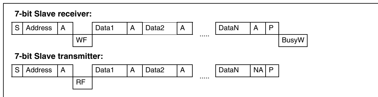
Figure 72. Transfer Sequencing
