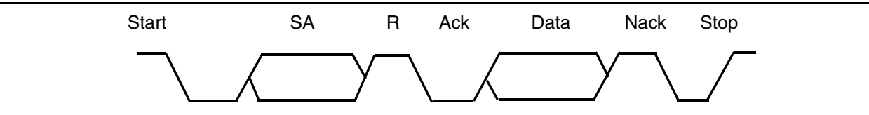
Figure 75. Current Address Read
