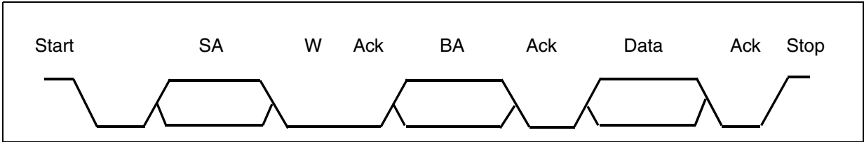
Figure 74. Page Write
