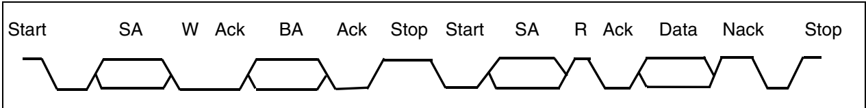
Figure 78. Sequential Read
