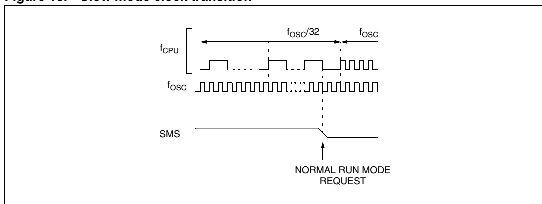
Figure 18. Slow mode clock transition
