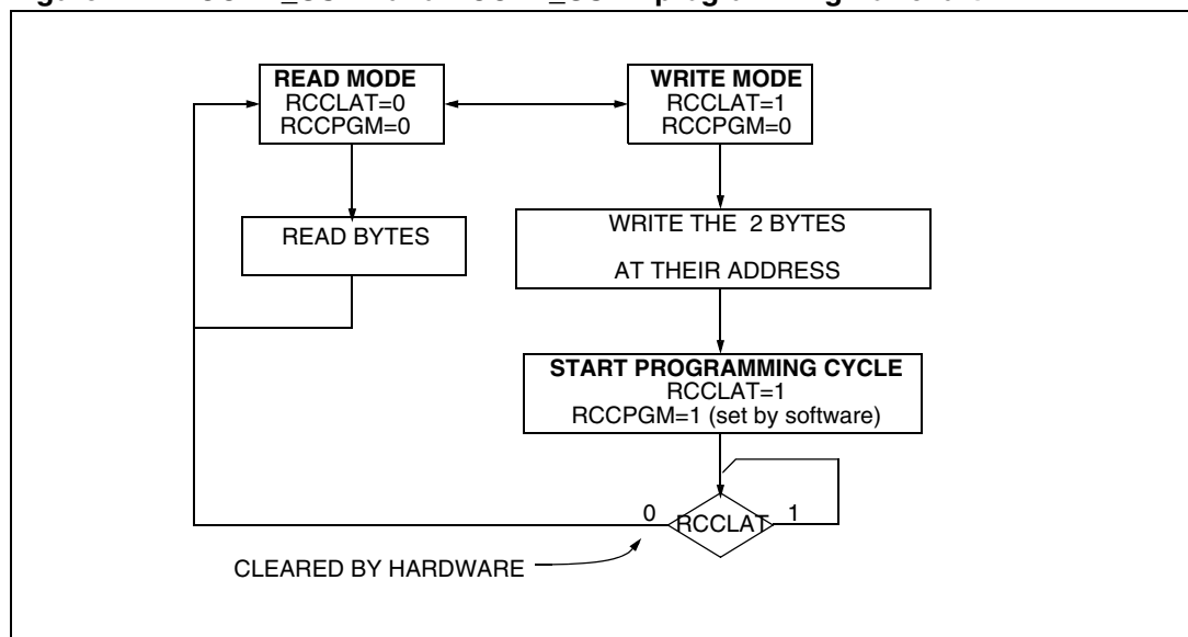
Figure 7. RCCR H _USER and RCCR L _USER programming flowchart
