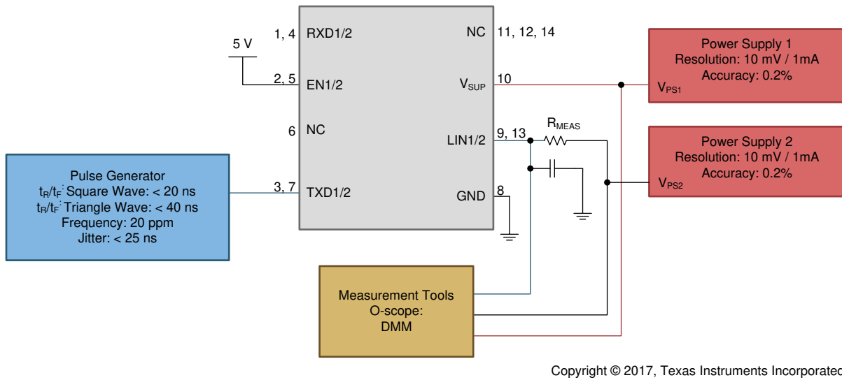
Figure 7-11. Test Circuit Slope Control and Duty Cycle Parameters 27, 28, 29, 30
