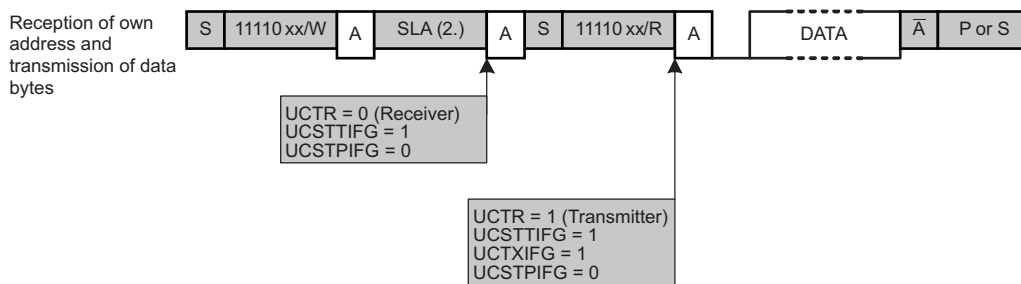
Figure 32-11. I 2 C Slave 10-Bit Addressing Mode
