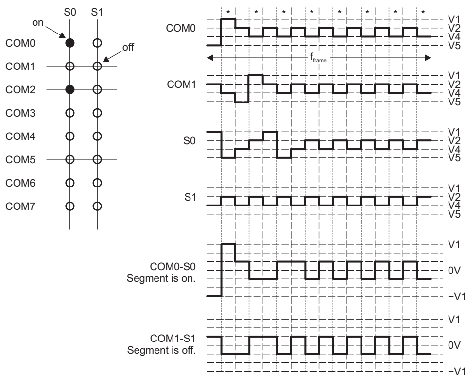
Figure 36-10. Example 8-Mux, 1/3 Bias Waveforms (LCDLP = 0)
