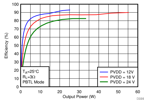
BD Modulation F SW = 768 kHz Load = 3 Ω PBTL Mode Figure 7-75. Efficiency vs Output Power
