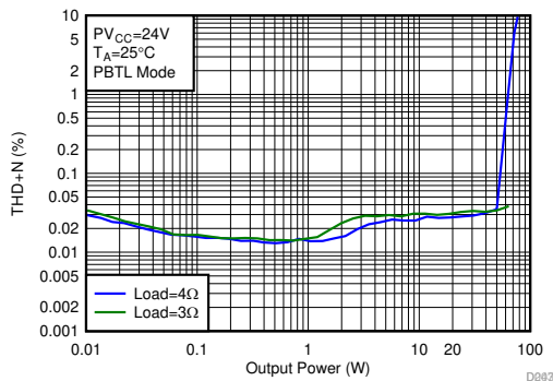
BD Modulation F SW = 768 kHz Load = 3 Ω, 4 Ω PBTL Mode Figure 7-72. THD+N vs Output Power-PBTL
