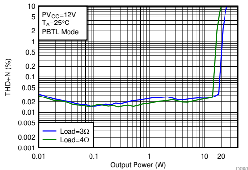
BD Modulation F SW = 768 kHz Load = 3 Ω, 4 Ω PBTL Mode Figure 7-70. THD+N vs Output Power-PBTL
