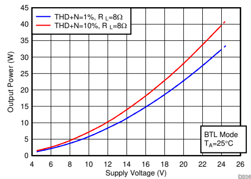
Figure 7-55. Output Power vs Supply Voltage
