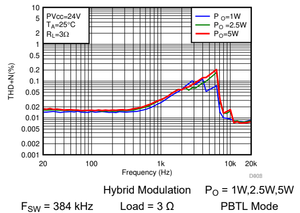
Figure 7-28. THD+N vs Frequency-PBTL
