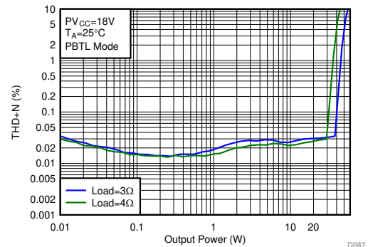
BD Modulation F SW = 768 kHz Load = 3 Ω, 4 Ω PBTL Mode Figure 7-71. THD+N vs Output Power-PBTL
