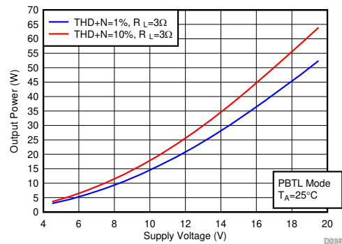
BD Modulation F SW = 768 kHz Load = 3 Ω PBTL Mode Figure 7-73. Output Power vs Supply Voltage
