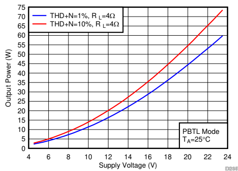
BD Modulation F SW = 768 kHz Load = 4 Ω PBTL Mode Figure 7-74. Output Power vs Supply Voltage
